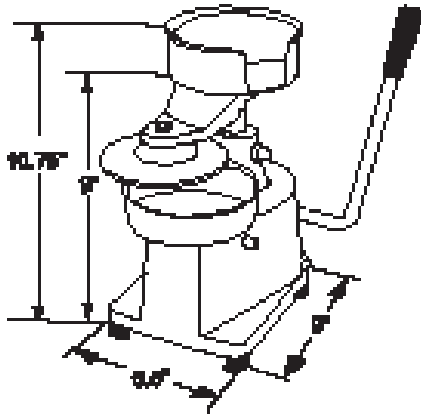
(21572 & 21573 Overall dimensions)
